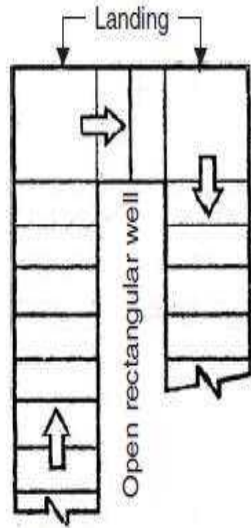
Fig. 8.37. Open well (newel) stair
